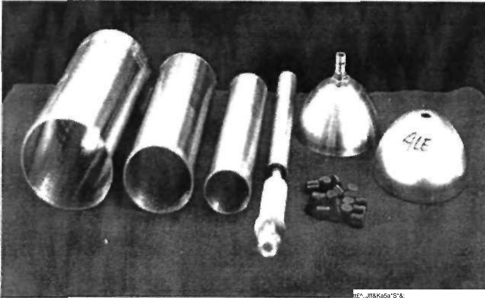
FIG 11. Cell - 4 cylinder. Cell parts show two types of domed tops. The little pile of ebonite spacers is shown near the two cones.
