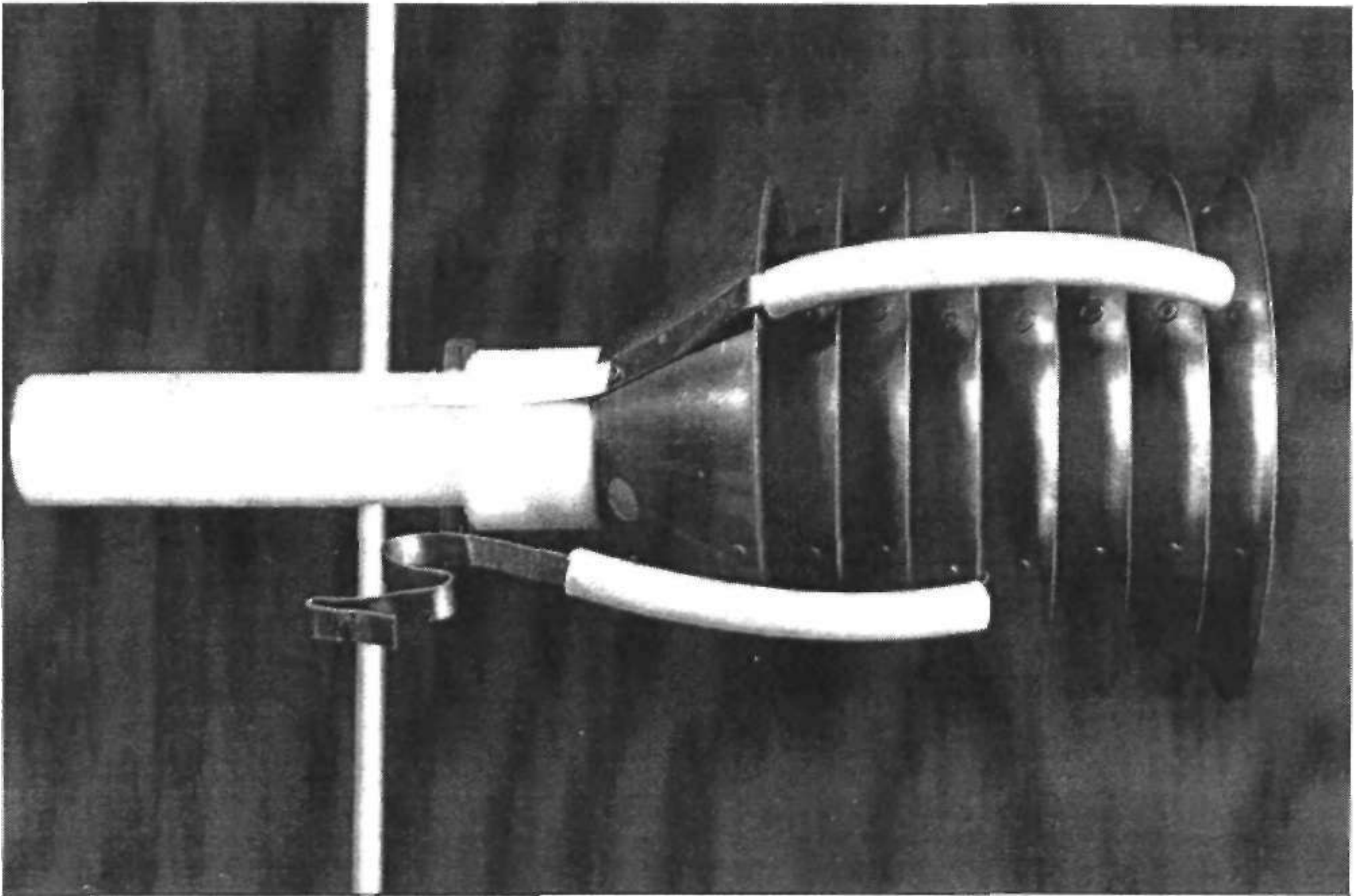
FIG 10. The Charging Vat. An overall view of the cone stack construction. Positive connection is the middle connection. Negative connections are to the second lowest and top cones.
