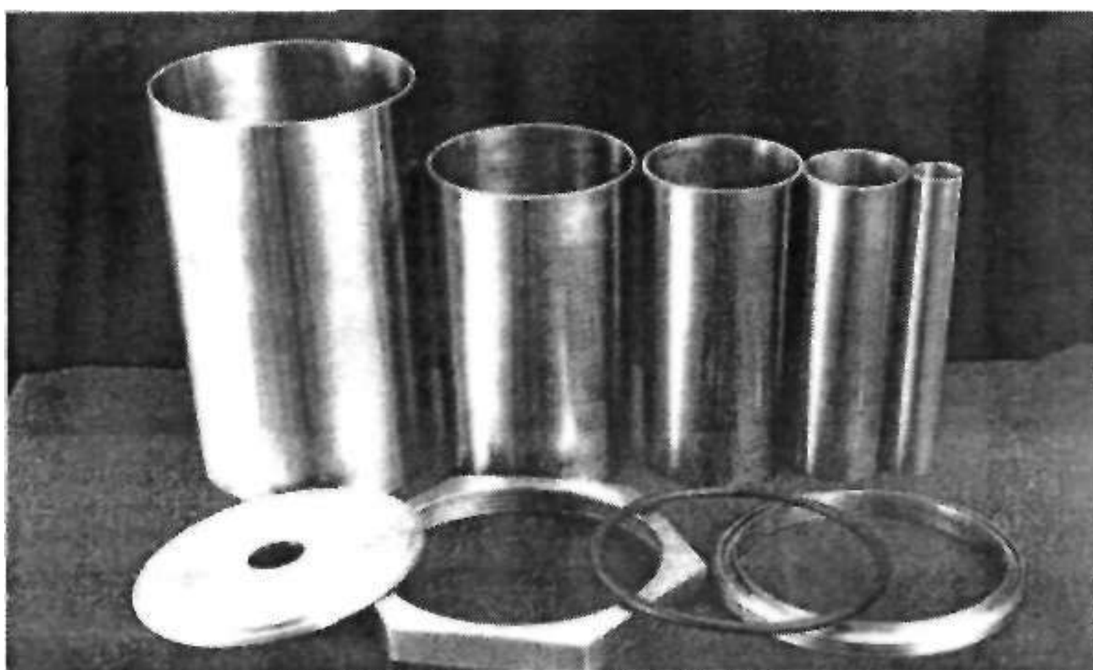
FIG 17. Cell - 5 cylinder. All major components of the cell. Note separate base plate and nut. The thread ring is still to be push fitted to the lower part of the outer cylinder.
