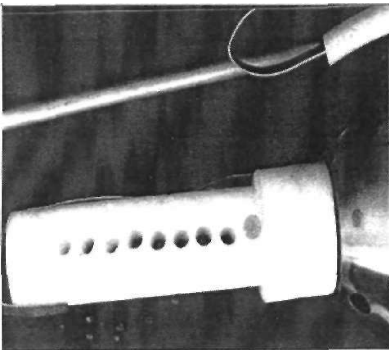
FIG 8. A side view of the central nylon rod showing the adjustment holes that allows a variable gap between the cone stack and the bottom of the vat.
