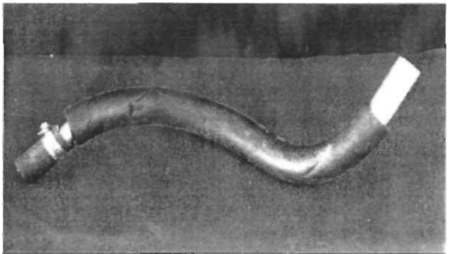
FIG 43. A view of the cell to engine connecting pipe . Notice that the blind plug end of the rubber tube does not have a hose fitting and thus would be a loose fit on the engine blind plug.
