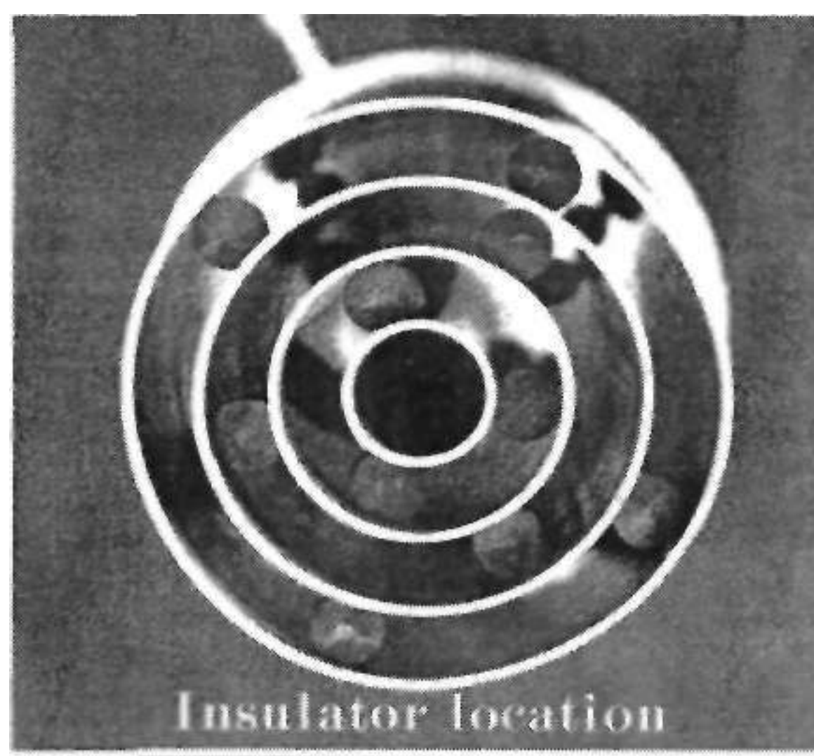
FIG 18. Cell - 4 cylinder. Position of ebonite spacer insulators. I use 3 insulators for the smaller cylinders and 4 for the larger cylinders. Insert at each end of the tubes.
