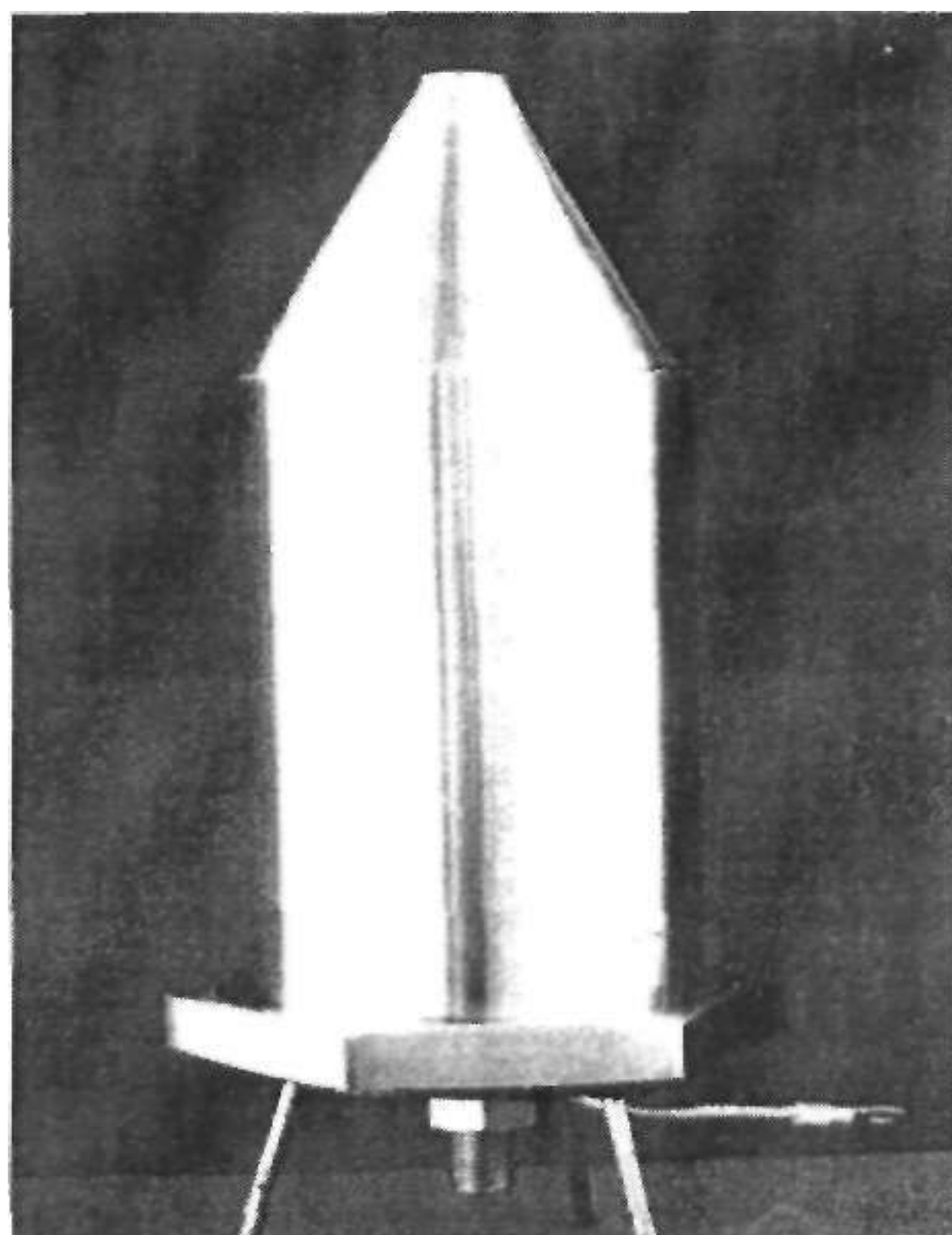
FIG 25. Cell - 5 cylinder. Completed cell. Notice the outlet compression fitting is missing
