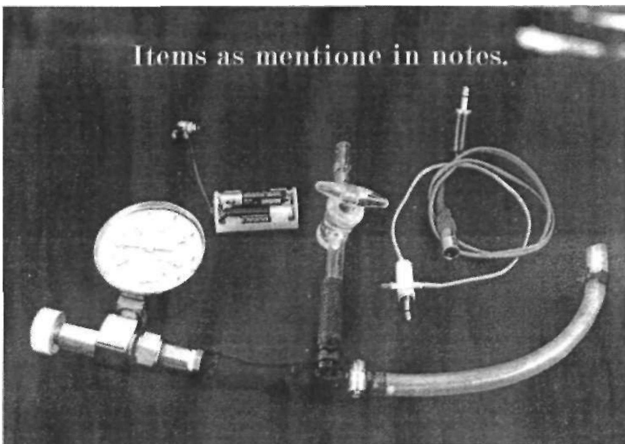
FIG 26. Useful tools - Test gauge reading pressure and vacuum, miniature light globe to observe action inside assembled cell and laser for observing particle sizes in the water.
