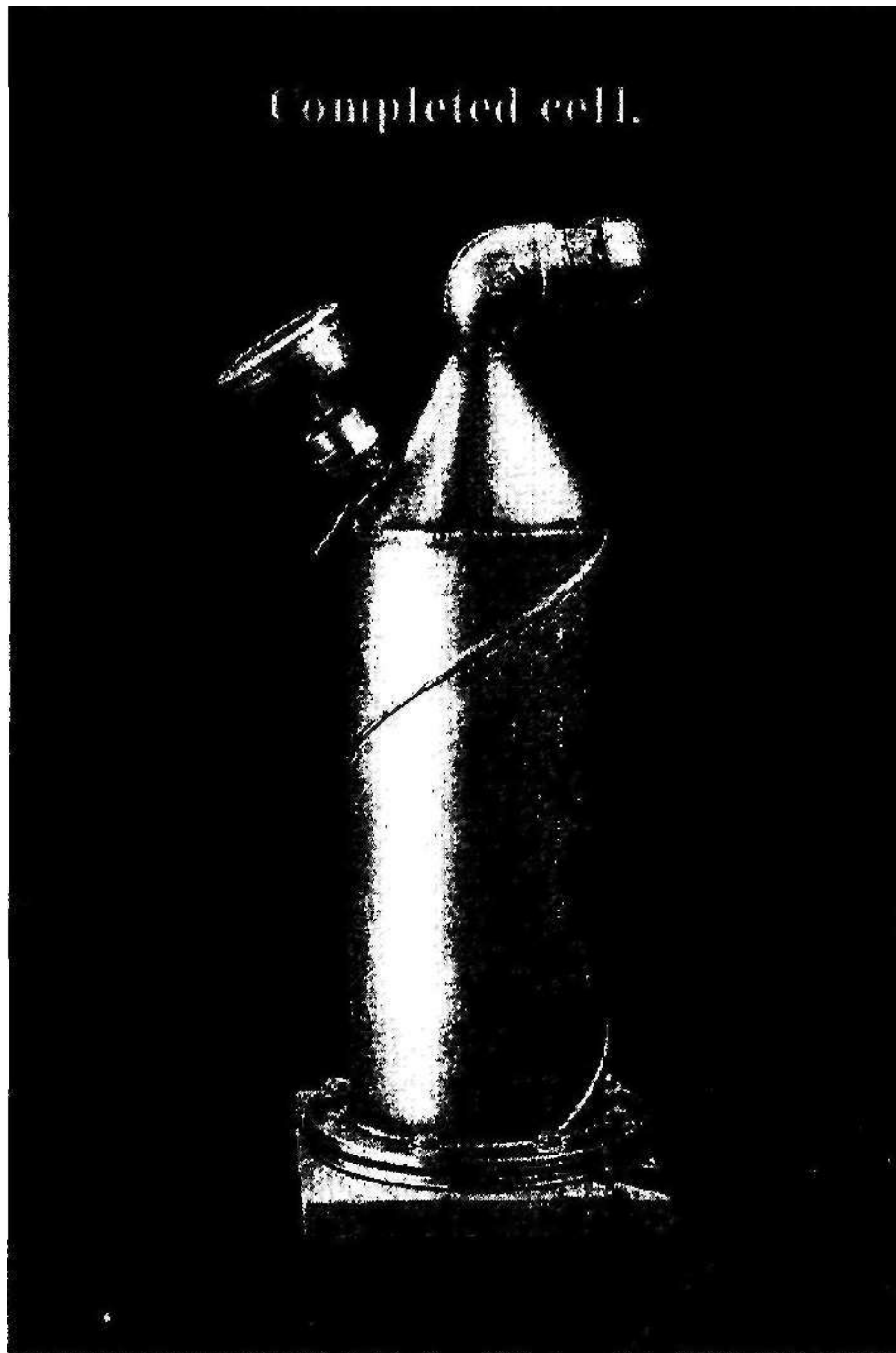
Fig. 1. - A view of "Old Trusty". A 3 year old cell that breaks most of the rules of cell design, but is still a great performer. The filling hole has a temporary pressure gauge fitted to monitor air leaks.
