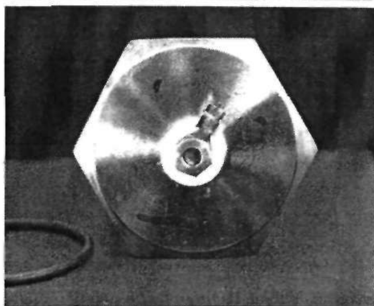
FIG 14. Cell - 4 cylinder. Showing the bottom cell cap completed with outer insulator and lug for the negative connection lead and fixing nut.
