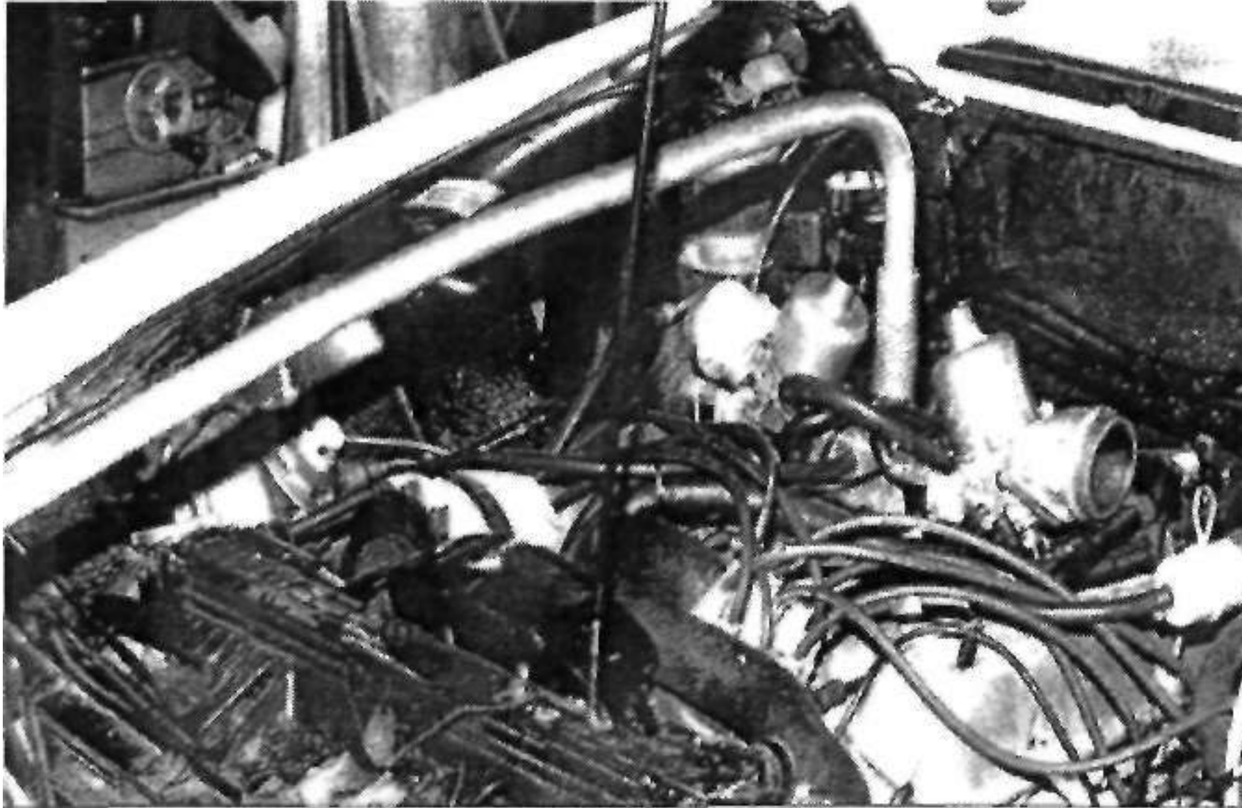
FIG 48. A view of the Rover engine used in the test set up showing the pipe extending from the external cell and connected to the inlet manifold. Notice downward angles on pipe and thus a compromise to the ideal
