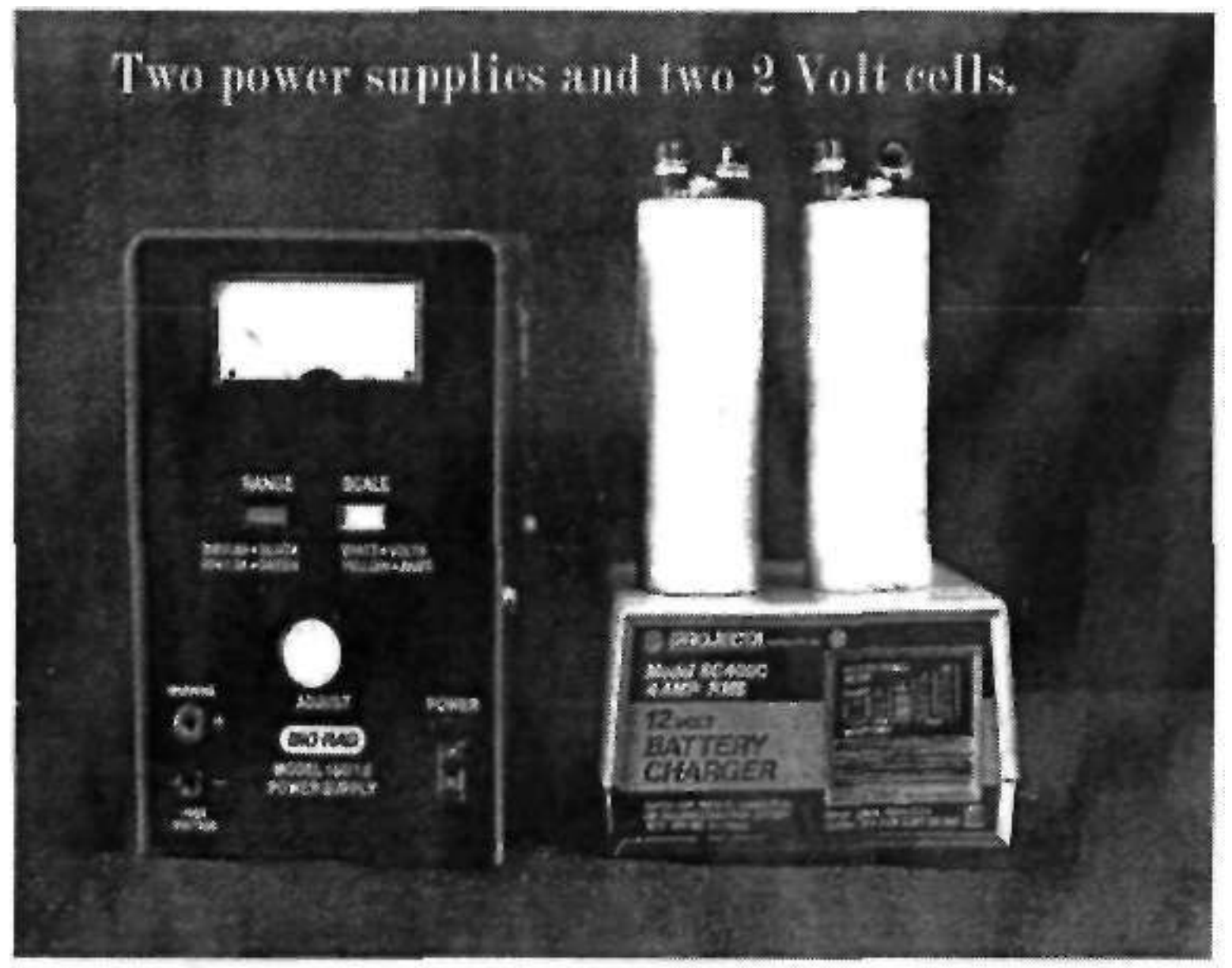
FIG 40. Left - view of a 60 Volt Charger for charging a cell without using electrolyte.
