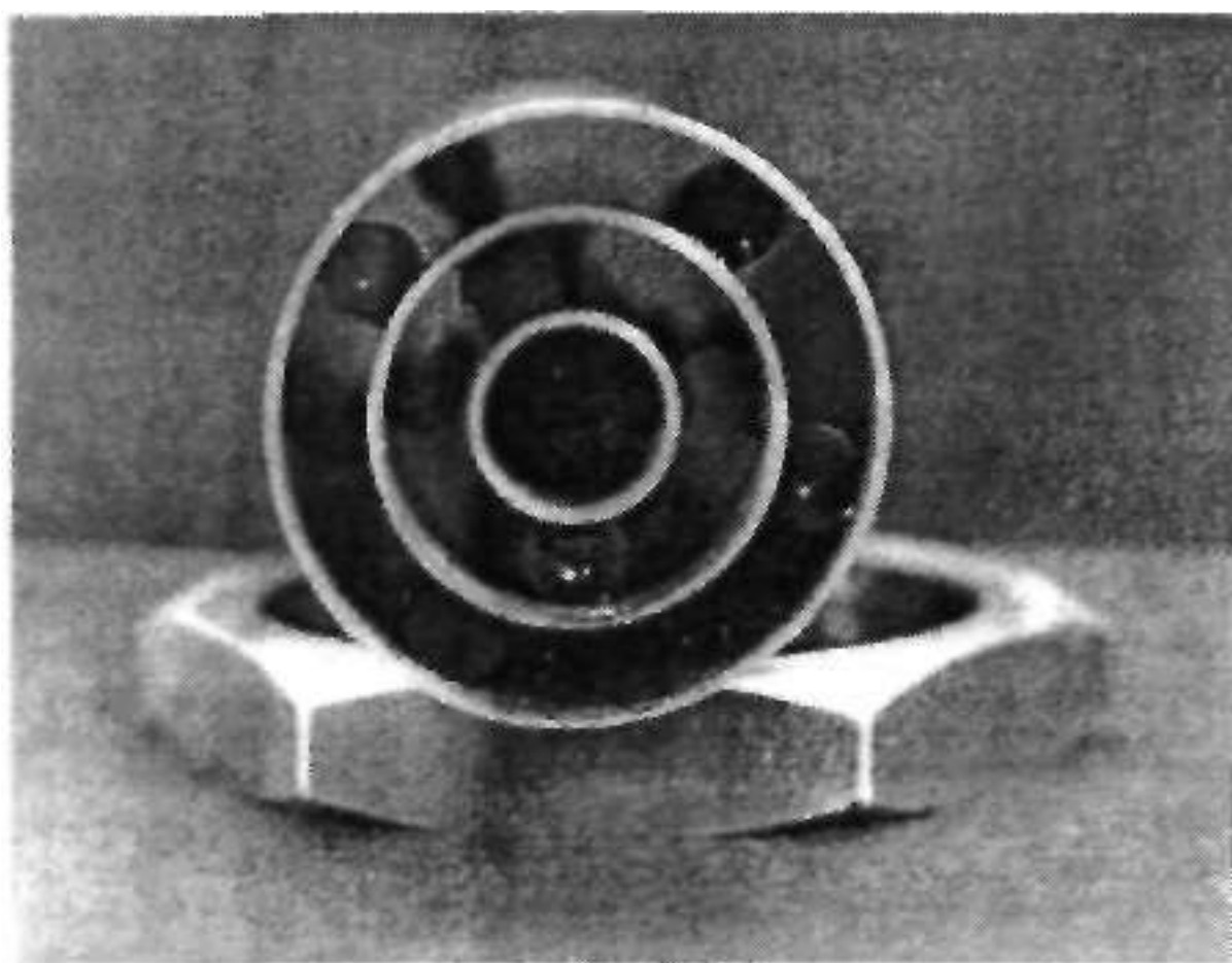
FIG 15. Cell - 4 cylinder. A view of the method for fitting the 1/2 inch long, 1/2 inch wide ebonite insulators
