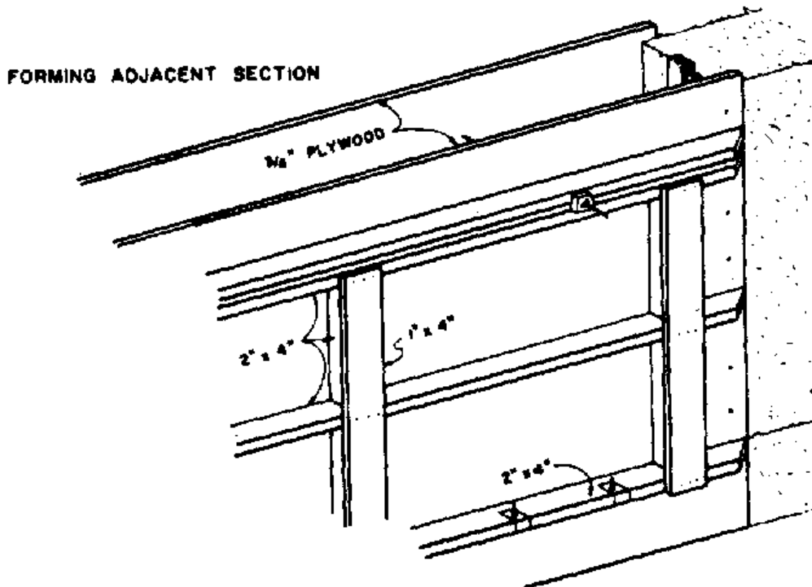
Figure 76. This is a special form that was designed to use the metal de strips shown in Figure 75.
