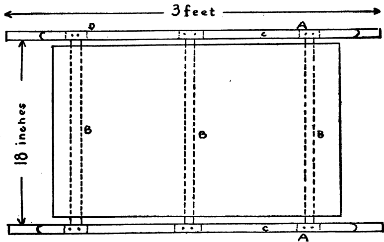
A ROCKABY COASTER
